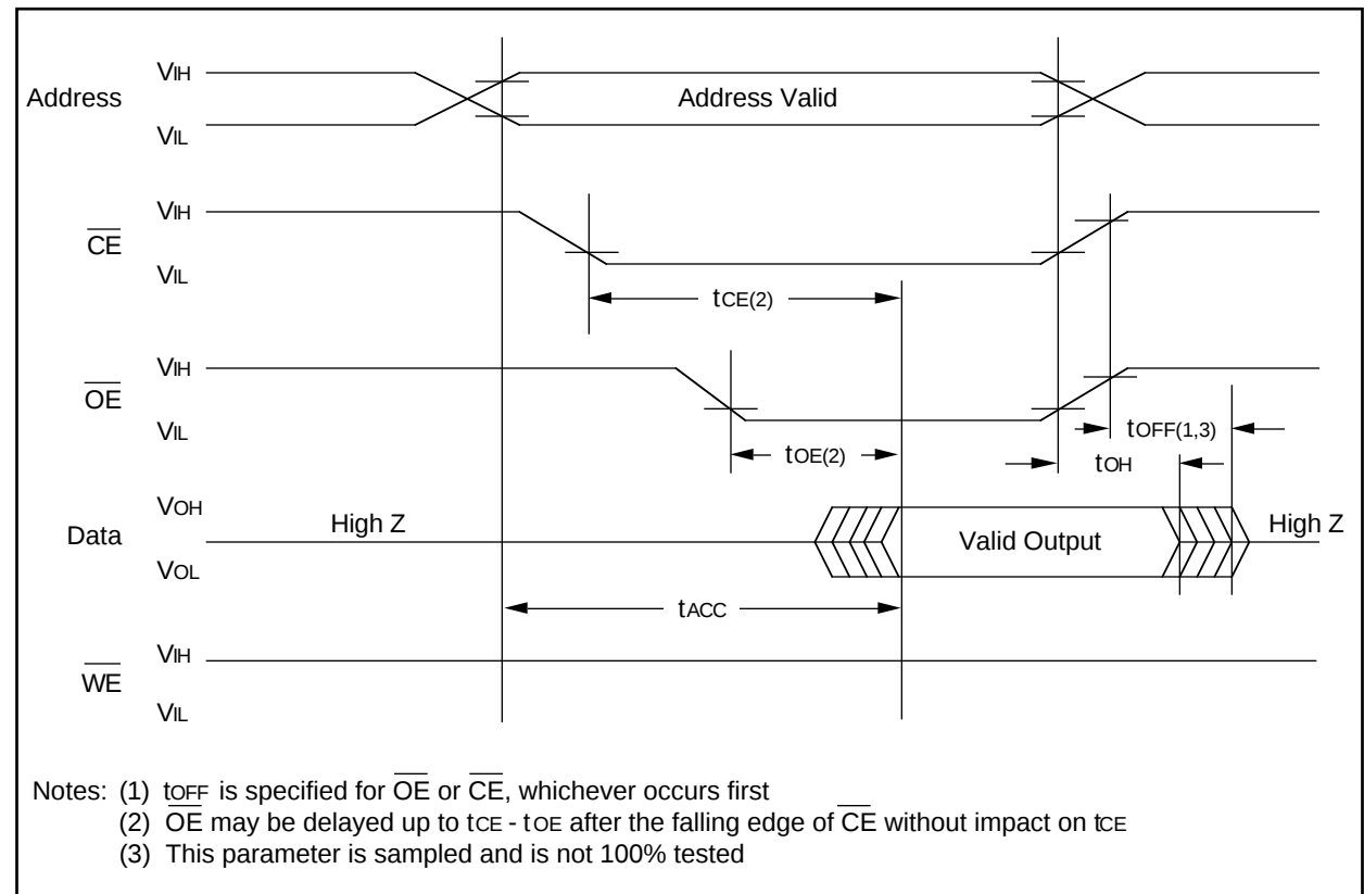
FIGURE 1-1: READ WAVEFORMS
