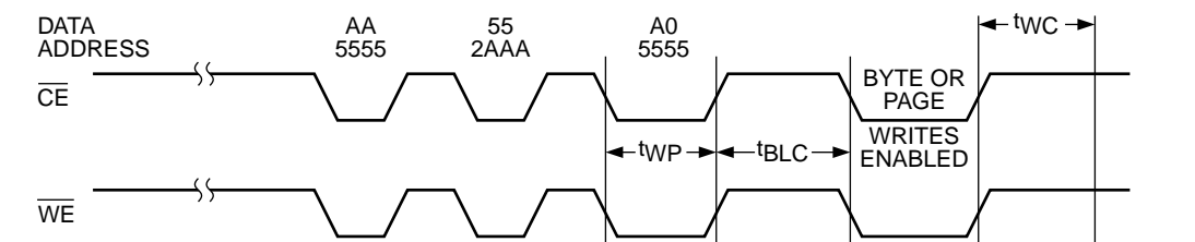
Figure 11. Software Data Protection Timing
